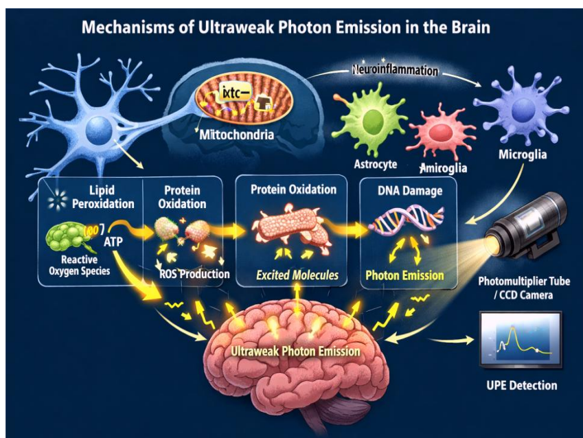
Figure 1: Basic Understanding of Mechanisms of Ultraweak Photon Emission in the Brain 26 (Image Source: GPT-5 mini, OpenAI, 2025). This diagram shows the cellular and molecular mechanisms involved in UPE in the brain tissue. The reactive oxygen species (ROS) are produced in the neurons and glial cells (astrocytes and microglia) by the mitochondrial oxidative metabolism. ROS interacts with lipids, proteins and DNA to generate electronically excited molecules. The relaxation of these molecules produces ultraweak photons (UPE), indicated by wavy arrows of yellow color. The intensity of photon emission can indicate neurophysiological processes, the role of glia and neuroinflammation. UPE is detected with sensitive optical sensors (i.e. photomultiplier tubes or charge-coupled device (CCD) cameras) which offer a possible non-invasive biomarker of brain oxidative stress and metabolic activity. Neurons: The main source of metabolic ROS because it is in high demand of ATP; oxidative byproducts of mitochondrial activity are associated with photon emission. Astrocytes and Microglia: Part of the oxidative metabolism and regulation of local UPE through neuroinflammatory signaling. ROS mediated processes: These processes are lipid peroxidation, protein oxidation, and DNA damage, and produce excited molecules that can emit photons. Photon Emission: The ultraviolet and visible spectrum (200-800 nm) of the light produce ultraweak photons that are emitted in the region that is significantly below the capability of human eyes to detect. Detection Systems: Photomultiplier tubes and CCD cameras can be used to quantify and spectrum analyse UPE and, thus, may be used to monitor potential metabolic and oxidative states.
